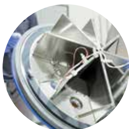
Propellant management devices: level gauges (liquid hydrogen and oxygen), anti-vortex
